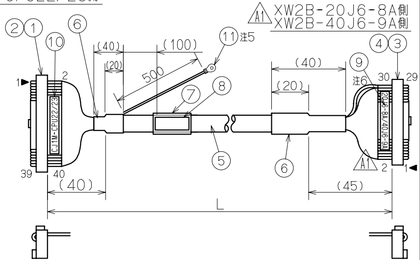
CJ1M-CPU22/23側
