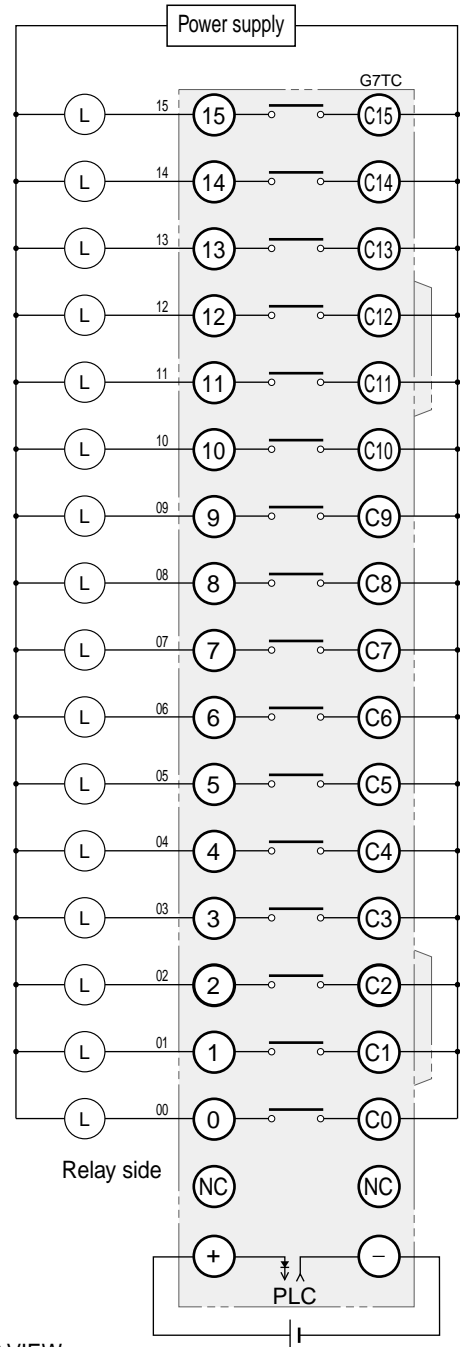
TOP VIEW
