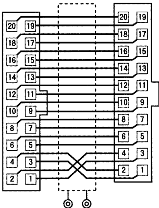
Wiring diagram
