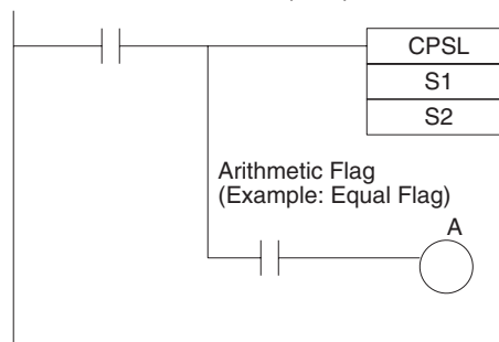
Correct Use of CPSL(115)
