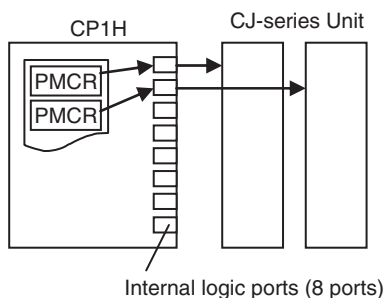
Internal logic ports (8 ports)
