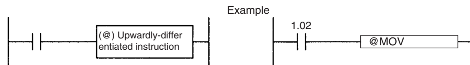
Executes the MOV instruction once when CIO 1.02 goes OFF → ON.
