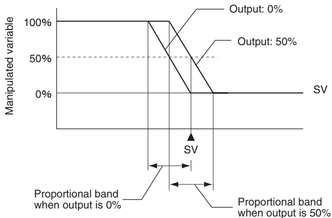
Proportional Action (Reverse Action)
