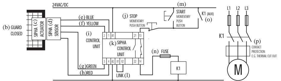
(q) Single sensor and single contactor. Machine will start when guard is closed and start button is pressed.
