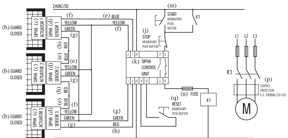
(u) Three sensors and one contactor with manual reset. Machine will start when all guards are closed, reset button is pressed and then start button is pressed. NOTE: The use of multiple sensors connected to a single control unit is only suitable in applications where each guard door is always opened and then shut individually. Otherwise single faults may not be detected and unintentional lockout reset may occur if two or more guard doors are open at the same time.
