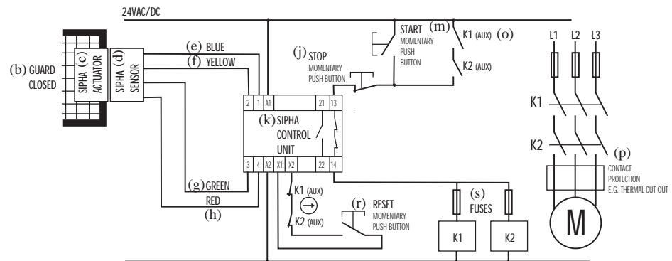
(t) Single sensor and two contactors with manual reset and contactor monitoring. Machine will start when guard is closed, auxiliary contacts at K1 & K2 are closed (i.e. both contactors are OFF), reset button is pressed and then start button is pressed.
