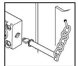
(g) Key C trapped, Key D free, guard open.
