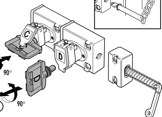
(g) Key C trapped, Key D free, guard open.
