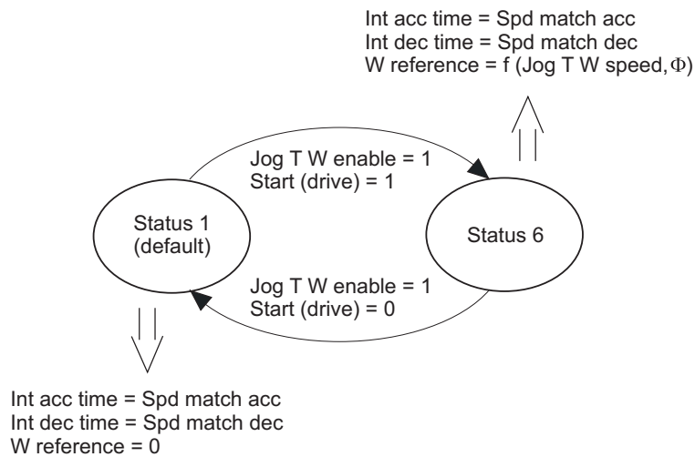
Figure 6.17.4: Functioning with Jog TW enable
