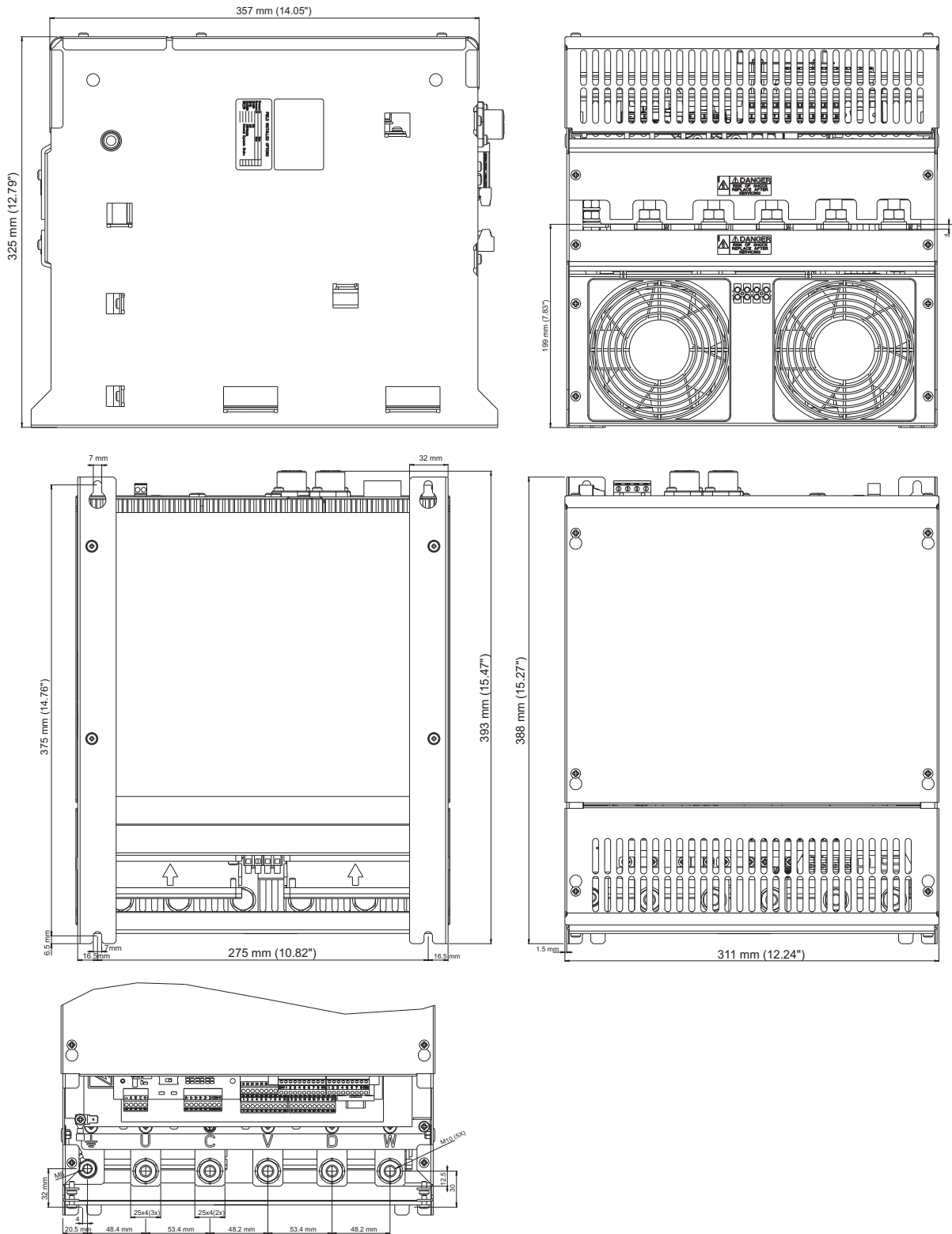
Fig. 2.5.3: Drive dimensions for 280 A ... 420 A sizes (form 2)
