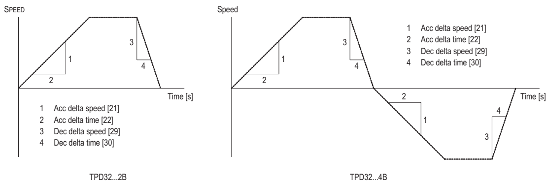
Figure 6.6.1.1: Accel, decel and Quick stop
