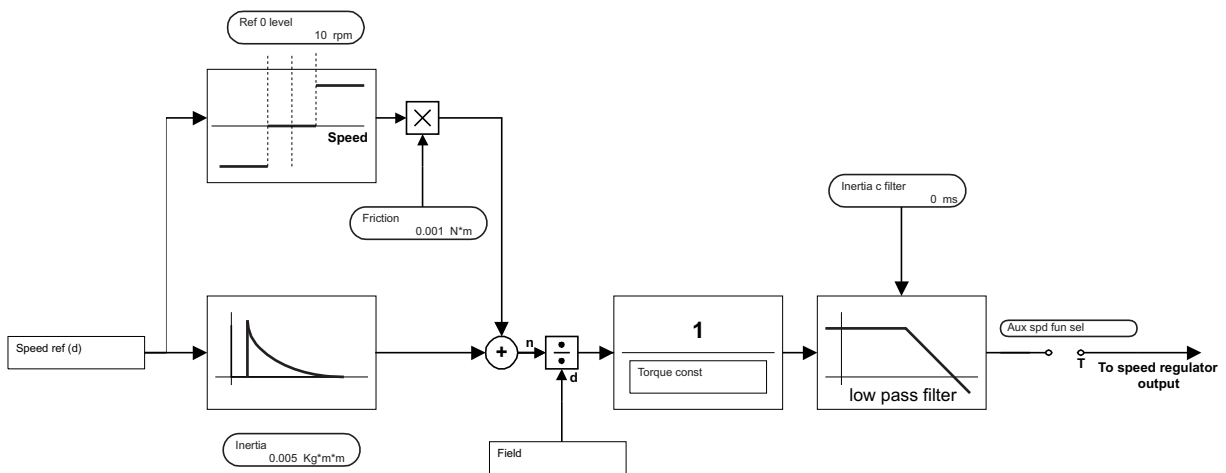
Figure 6.7.5.1: Inertia/Loss compensation
