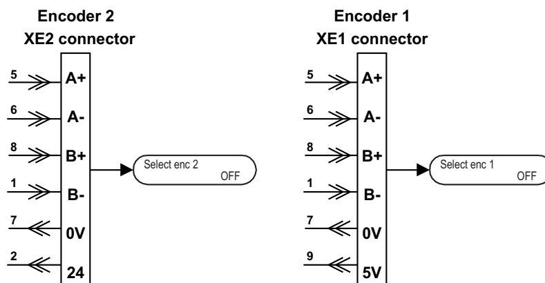
Figure 6.12.5.1: Tach follower
