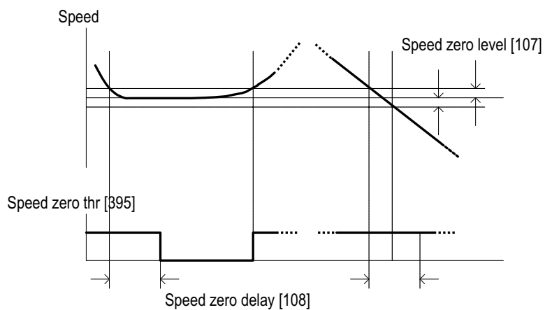
Figure 6.13.4.1: Speed zero
