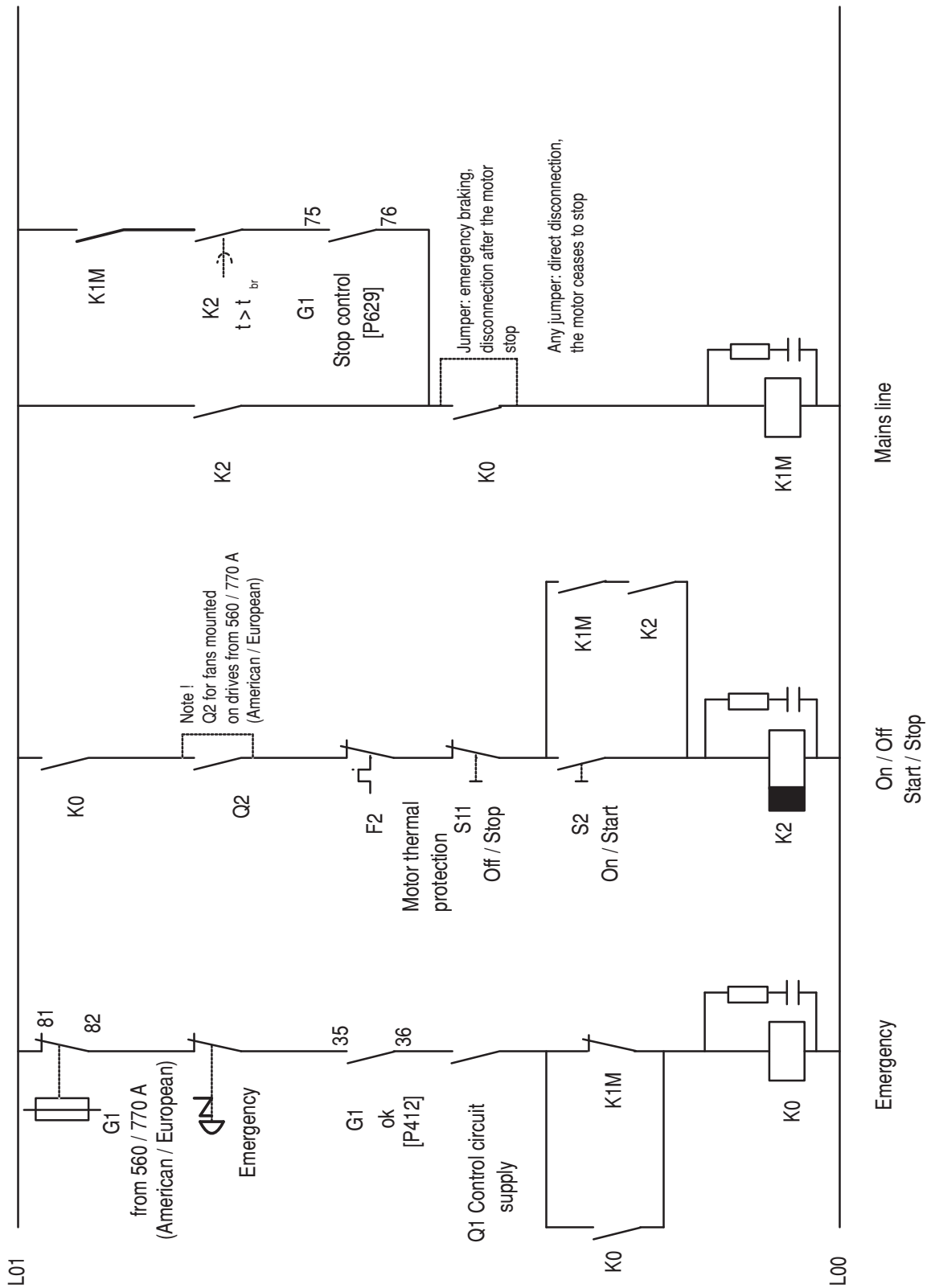
Figure 4.8.1: Control sequencing
