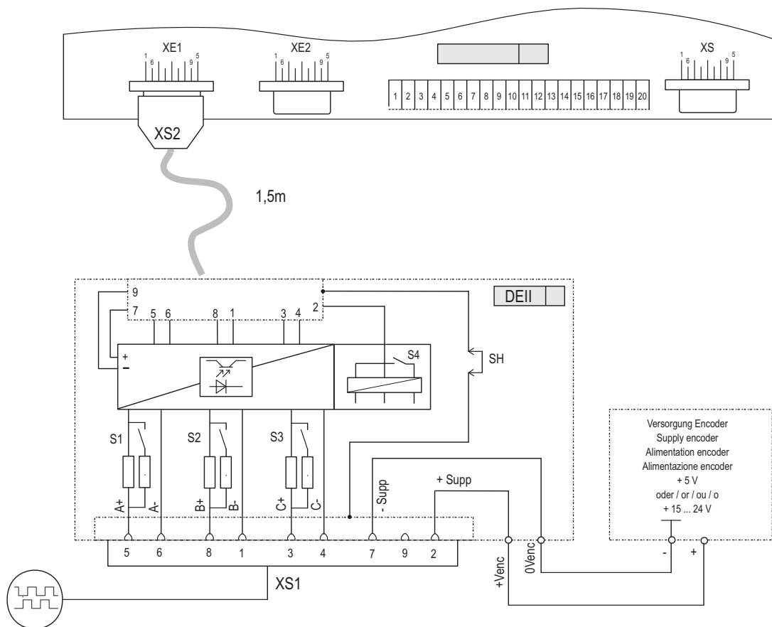
Figure 4.8.7: DEII connection
