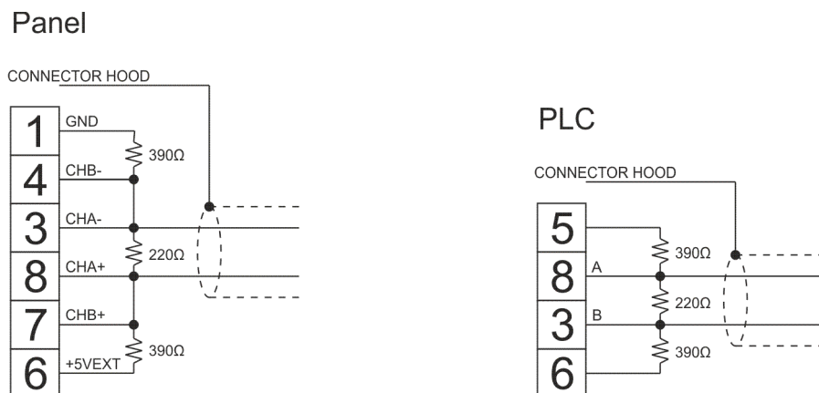
Figure 2. Termination resistors
