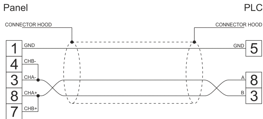
Figure 1. Cable diagram
