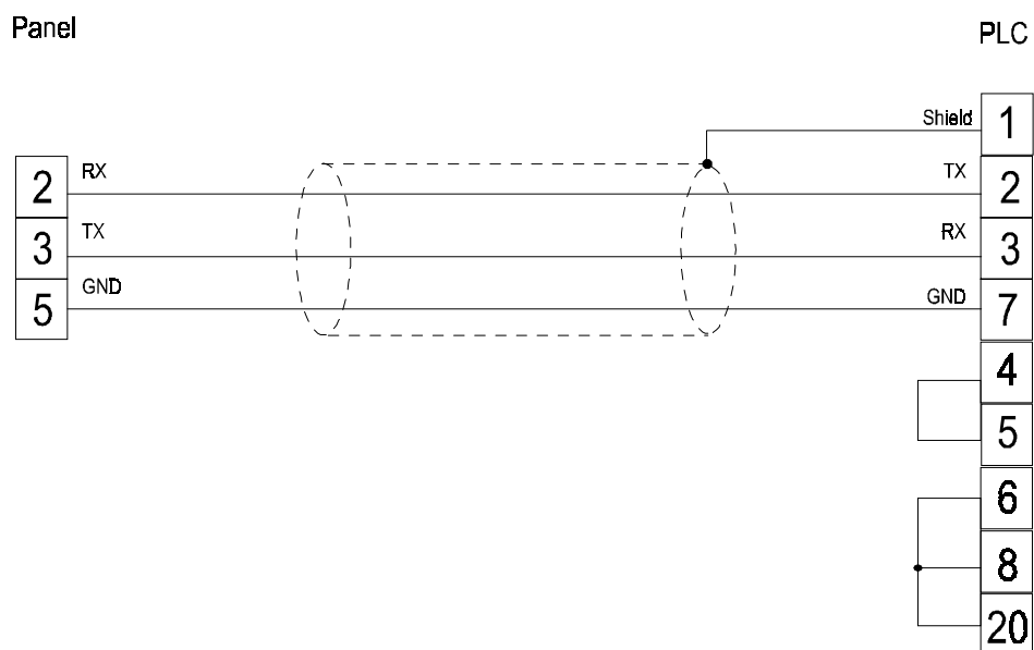
figure 1. Cable diagram
