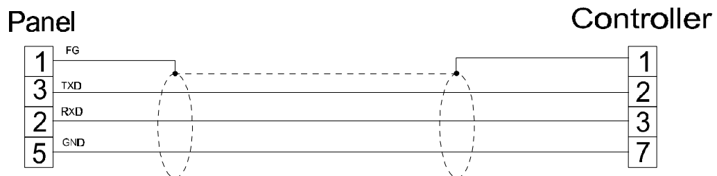
Figure 1. Cable diagram
