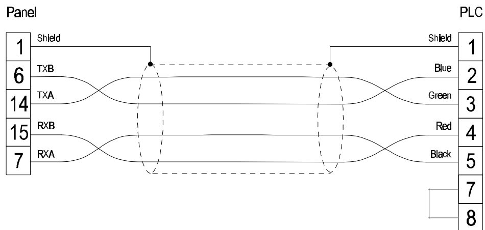
Figure 1. Cable diagram
