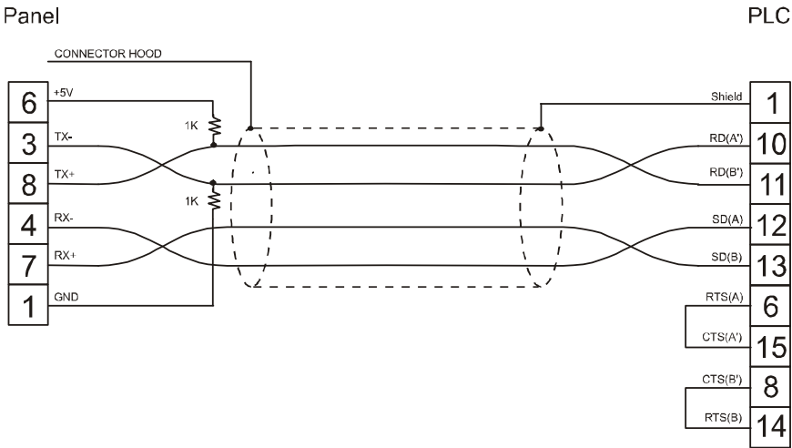
figure 1. Cable diagram
