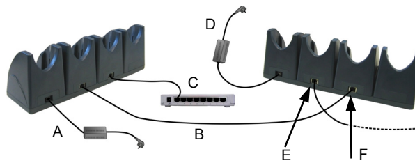
Figure 4 - Daisy chaining Ethernet Connection
