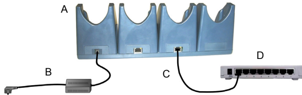
Figure 3 - Ethernet Connection
