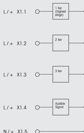
Connection diagram
