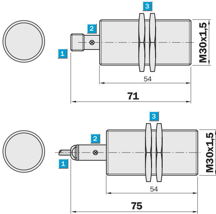
Dimensional drawing
