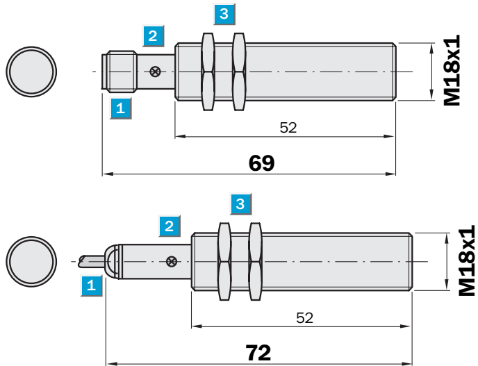
Dimensional drawing
