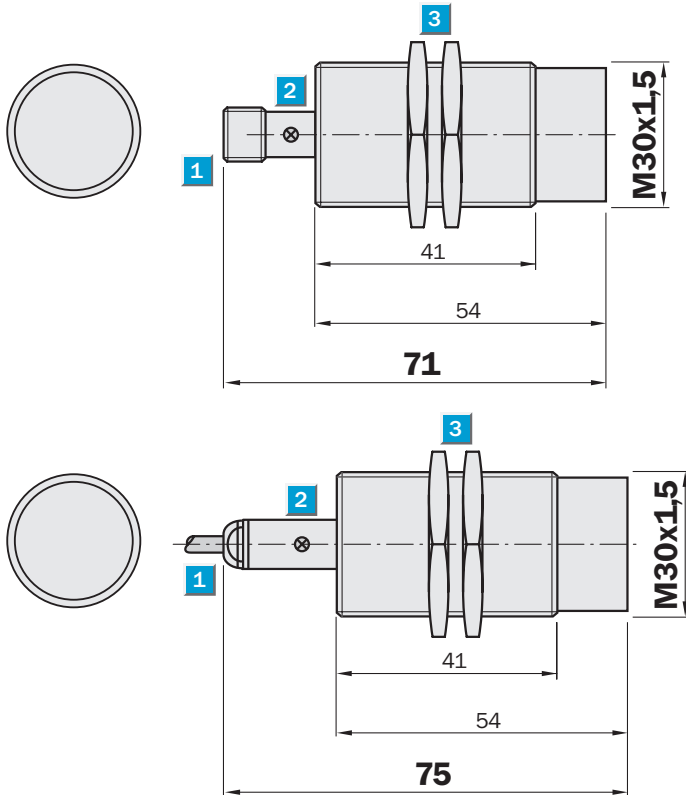
Dimensional drawing
