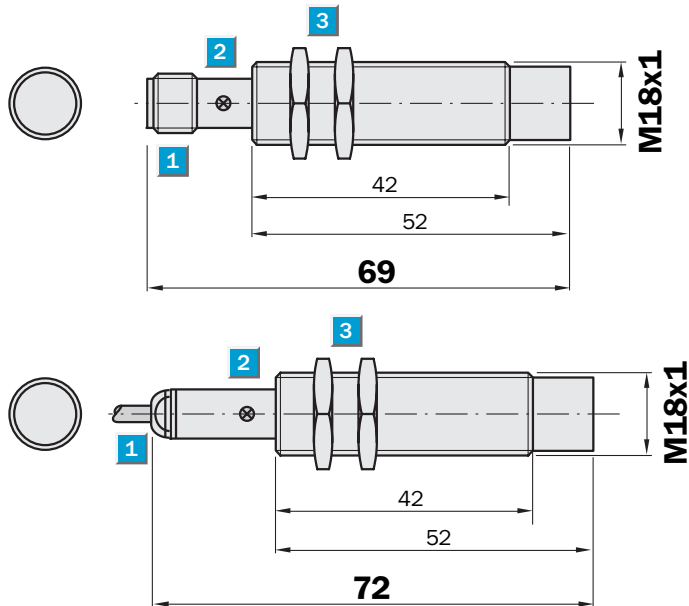
Dimensional drawing
