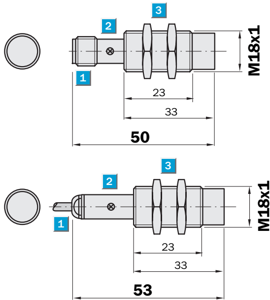
Dimensional drawing
