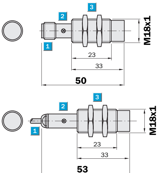
Dimensional drawing
