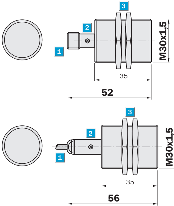
Dimensional drawing
