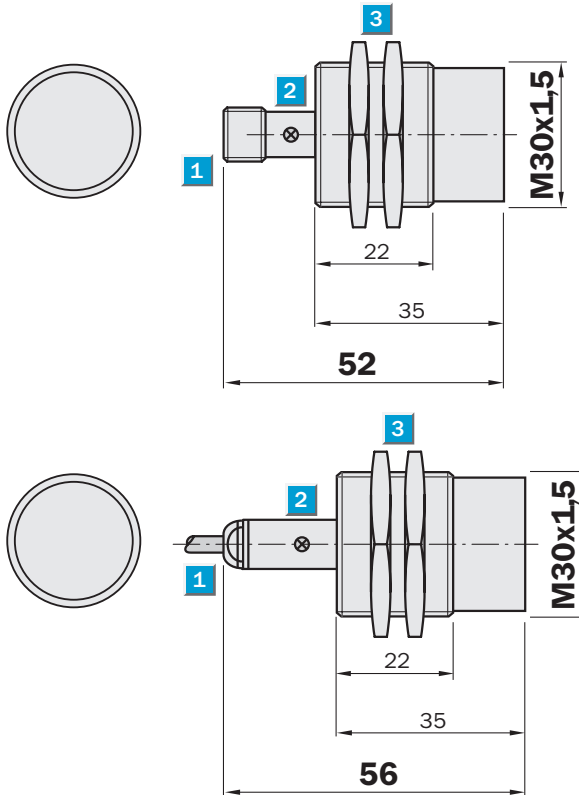
Dimensional drawing
