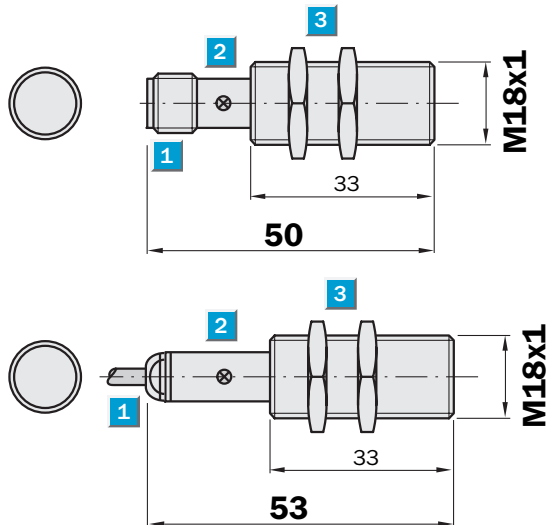
Dimensional drawing
