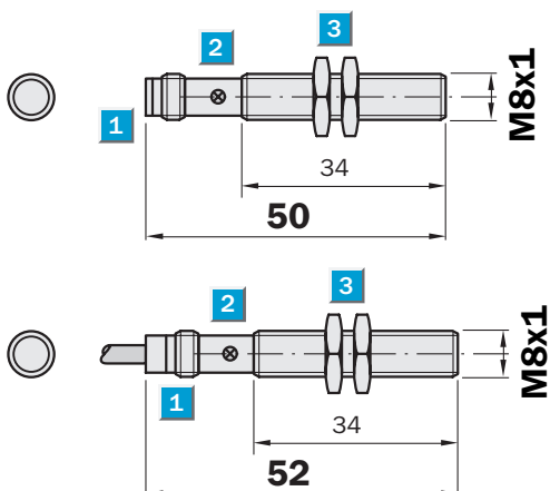
Dimensional drawing
