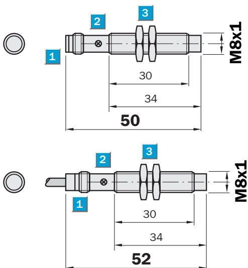
Dimensional drawing
