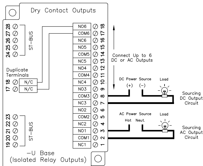
Equivalent Circuit
