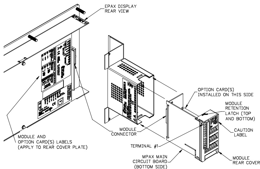
Figure 1, Installing an MPAX Module and Option Cards
