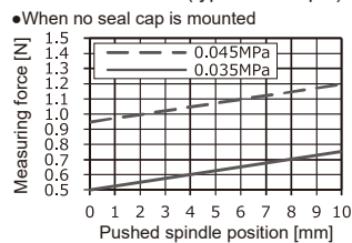
<Downward mount (typical example)> •When no seal cap is mounted
