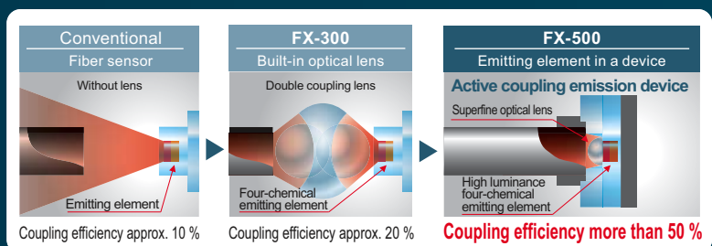
Coupling efficiency \approx (light intensity directed into the fiber / emission intensity of active coupling emission device) \times 100 * Illustration is an image.
