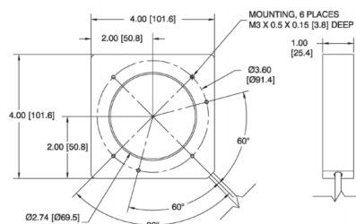
Smart Series R-100 Ring Light Dimensions
