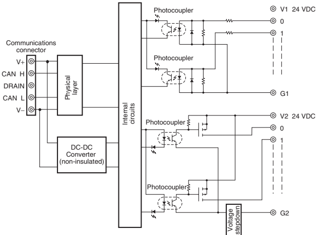
DRT2-MD16-1 (PNP)
