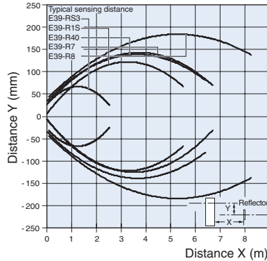
Retro-reflective Models E3F2-R4□4-□
