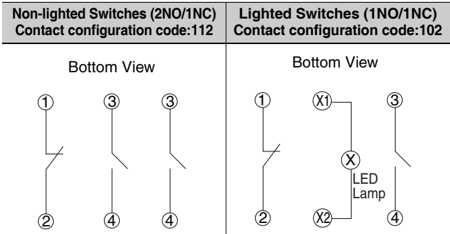
Terminal Connection Diagrams
