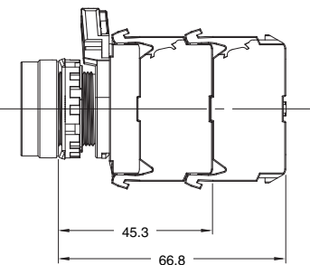
Depth with Linked Units (Screw terminal block type)
