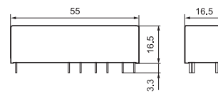
Type 50.16
