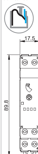
Type 14.61 Bornes Push-in
