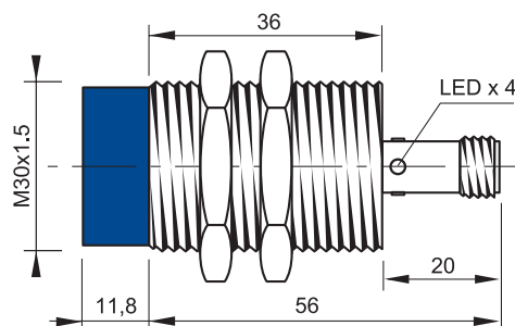
CONFIGURATION WITH CONNECTOR M12
