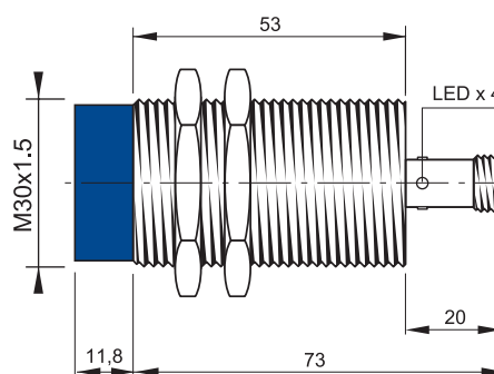
CONFIGURATION WITH CONNECTOR M12
