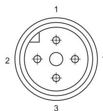
View of quadripole male connector
