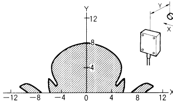
V600-HS61 + V600-D8KR12
