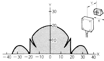
V600-HS63 + V600-D23P71
