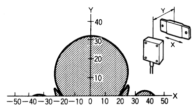
V600-HS63 + V600-D8KR12
