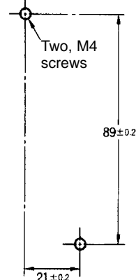
Mounting Hole Dimensions
