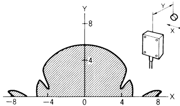
V600-HS61 + V600-D23P72
