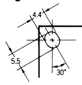
Enlargement of Mounting Hole
