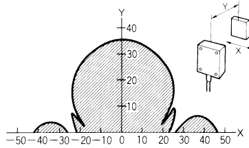
V600-HS63 + V600-D23P72
