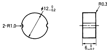
V600-D23P54 Data Carrier
