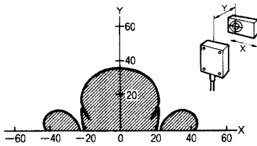
V600-HS63 + V600-D8KR13
