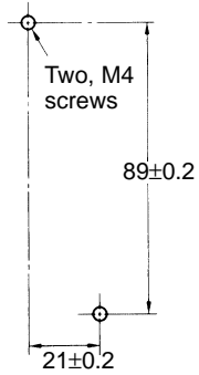
Mounting Hole Dimensions
