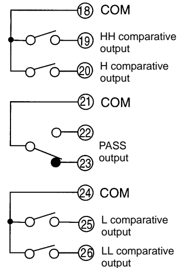
K3NX with 5 Relay Output Boards, K31-C5
