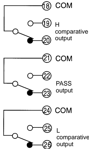
K3NX with 5 Relay Output Boards, K31-C5
