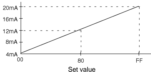
4 to 20 mA outputs
