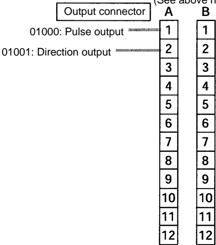
Pulse + Direction Outputs (See above note.)
