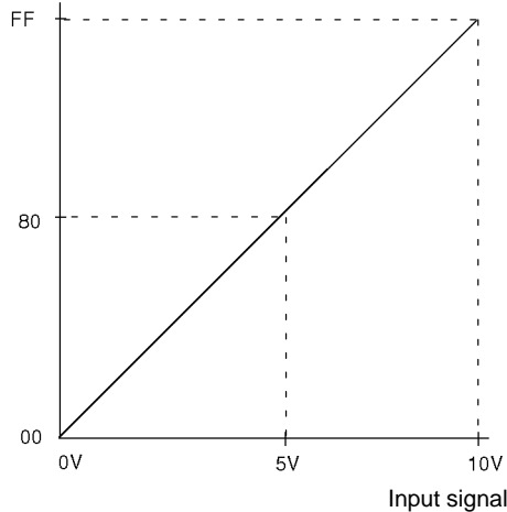
0 to 10 V inputs Conversion value
