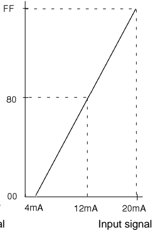
4 to 20 mA inputs Conversion value
