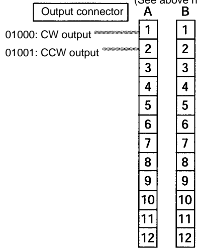
Up/down Pulse Outputs (See above note.)
