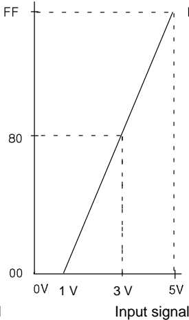
1 to 5 V inputs Conversion value
