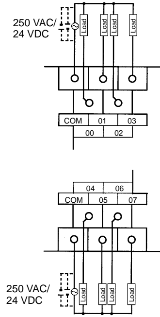
CPM1A-8ER
