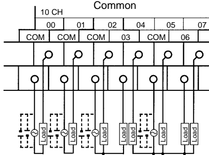
CPM1A-20CDR-□(-V1)/CPM1A-20EDR/20EDR1
