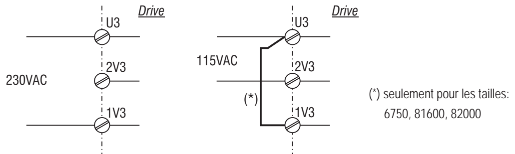
Figure 4.2.3: Raccordement extérieur
