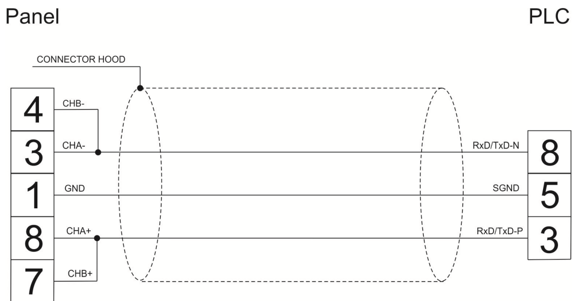
Figure 1. Cable diagram
