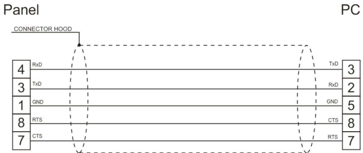
figure 1. Cable diagram
