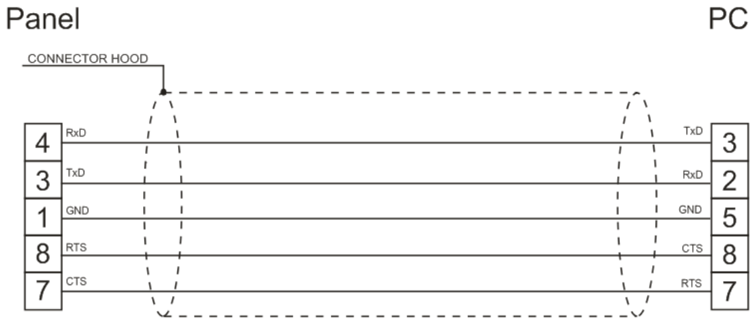
figure 1. Cable diagram
