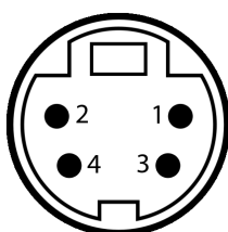
Figure 2. PLC connector (Male - Frontal View)
