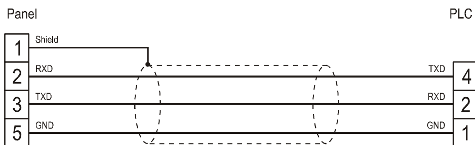
Figure 1. Cable diagram
