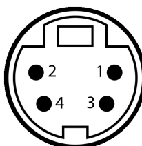
Figure 2. PLC connector (Male - Frontal View)
