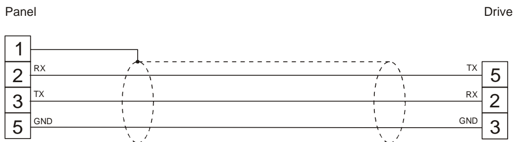
figure 1. Cable diagram
