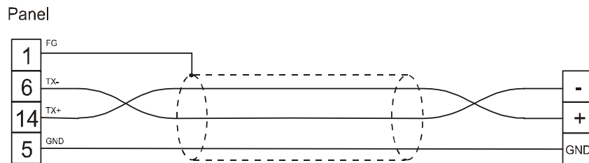
Figure 1. Cable diagram
