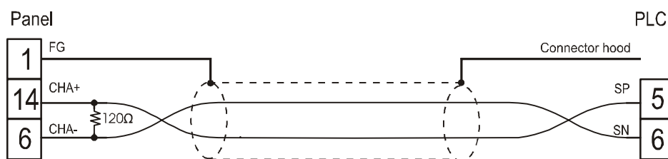
Figure 1. Cable diagram
