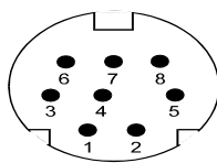
figure 2. Connector front view (pin side)
