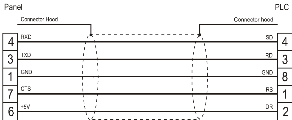
Figure 1. Cable diagram
