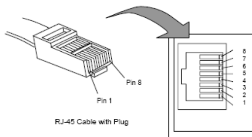
Figure 2. PLC Connector
