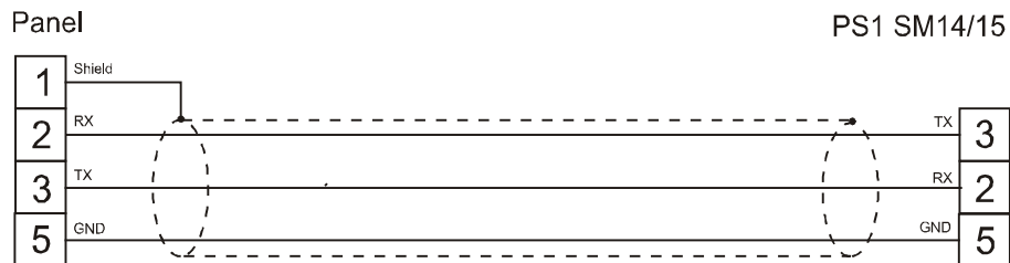
figure 1. Cable diagram
