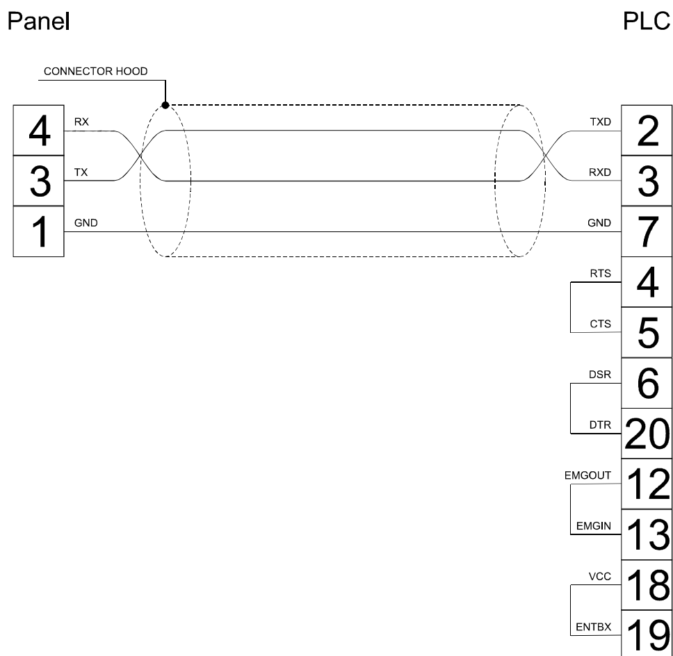
figure 1. Cable diagram
