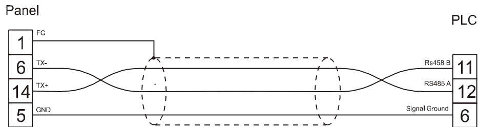
figure 1. Cable diagram
