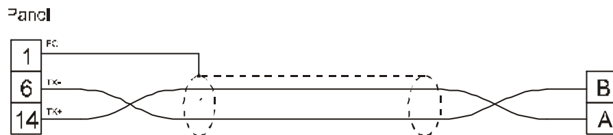
figure 1. Cable diagram
