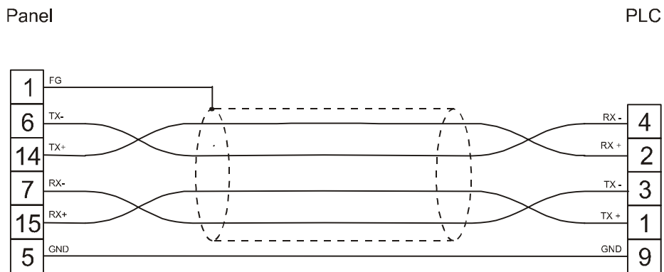
figure 1. Cable diagram
