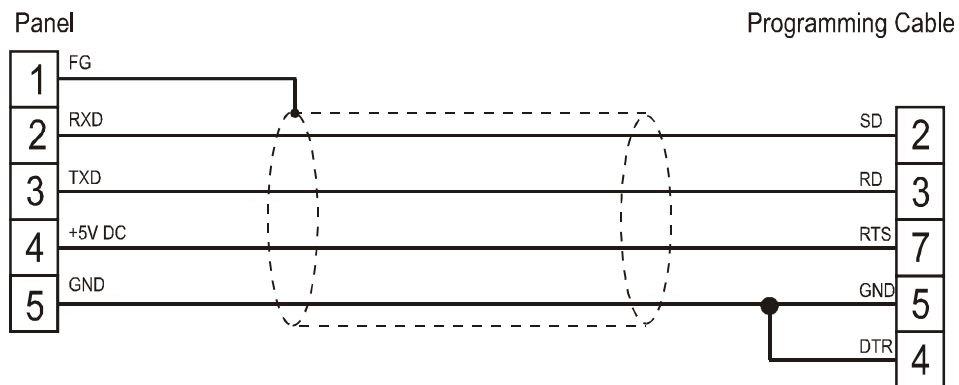
Figure 1. Cable diagram
