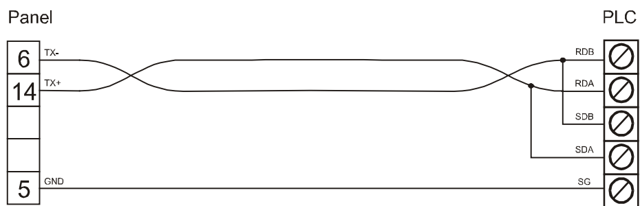
figure 1. Cable diagram
