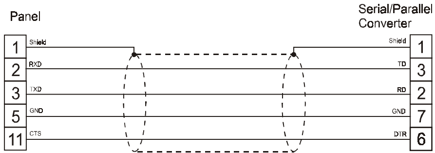
figure 1. Cable diagram
